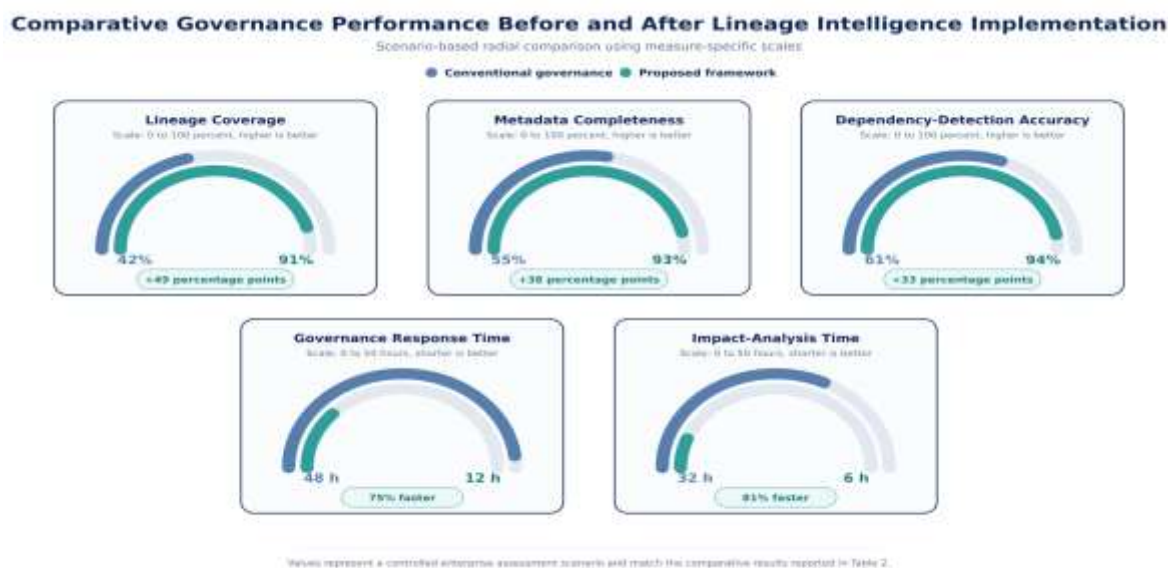
Figure 6. Comparative Governance Performance Before and After Lineage Intelligence Implementation
