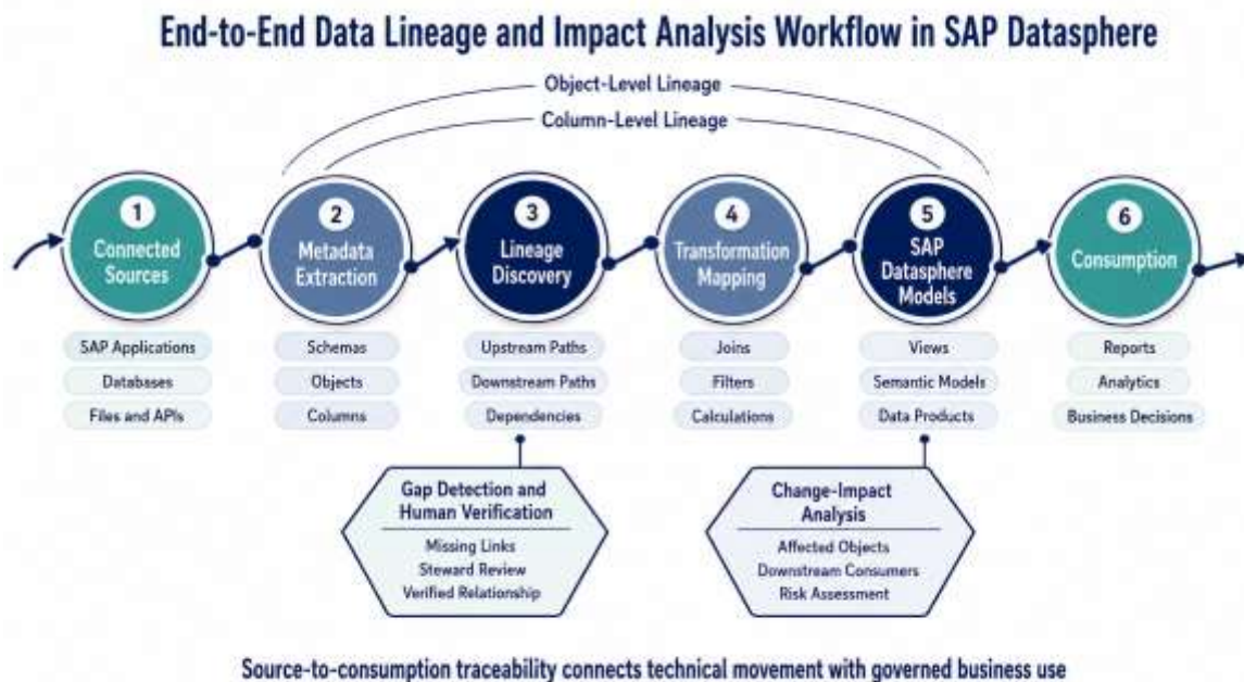
Figure 4. End-to-End Data Lineage and Impact Analysis Workflow in SAP Datasphere
