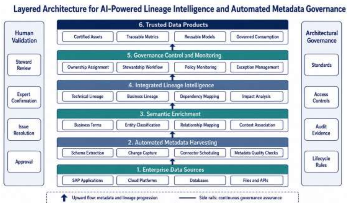
Figure 3. Layered Architecture for AI-Powered Lineage Intelligence and Automated Metadata Governance
